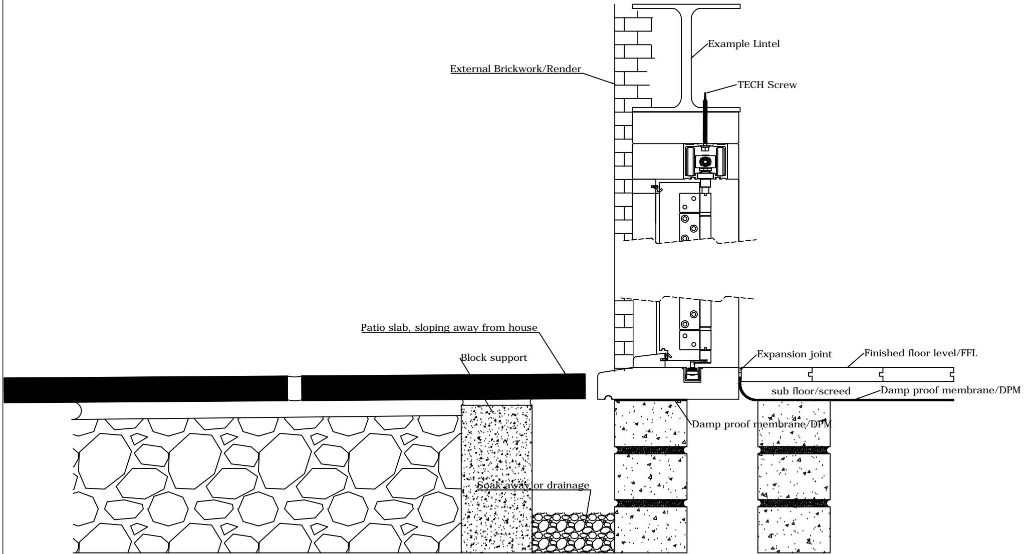
Valdi Ltd - Top Hung Folding Sliding Doors - Standard Timber Drip Sill - Inward opening - Raised Patio Construction
